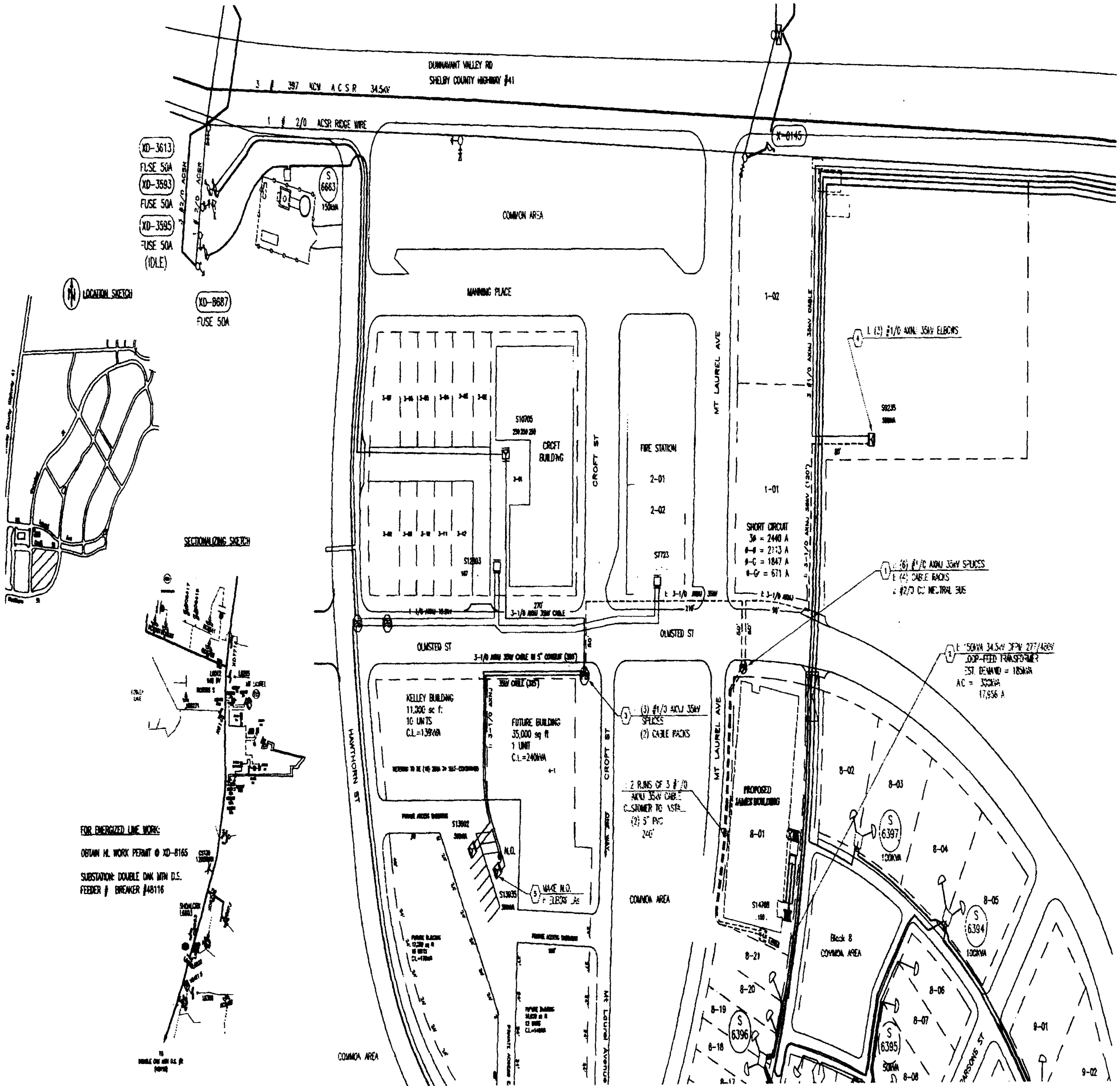
PULLING @ LOCATION 15
