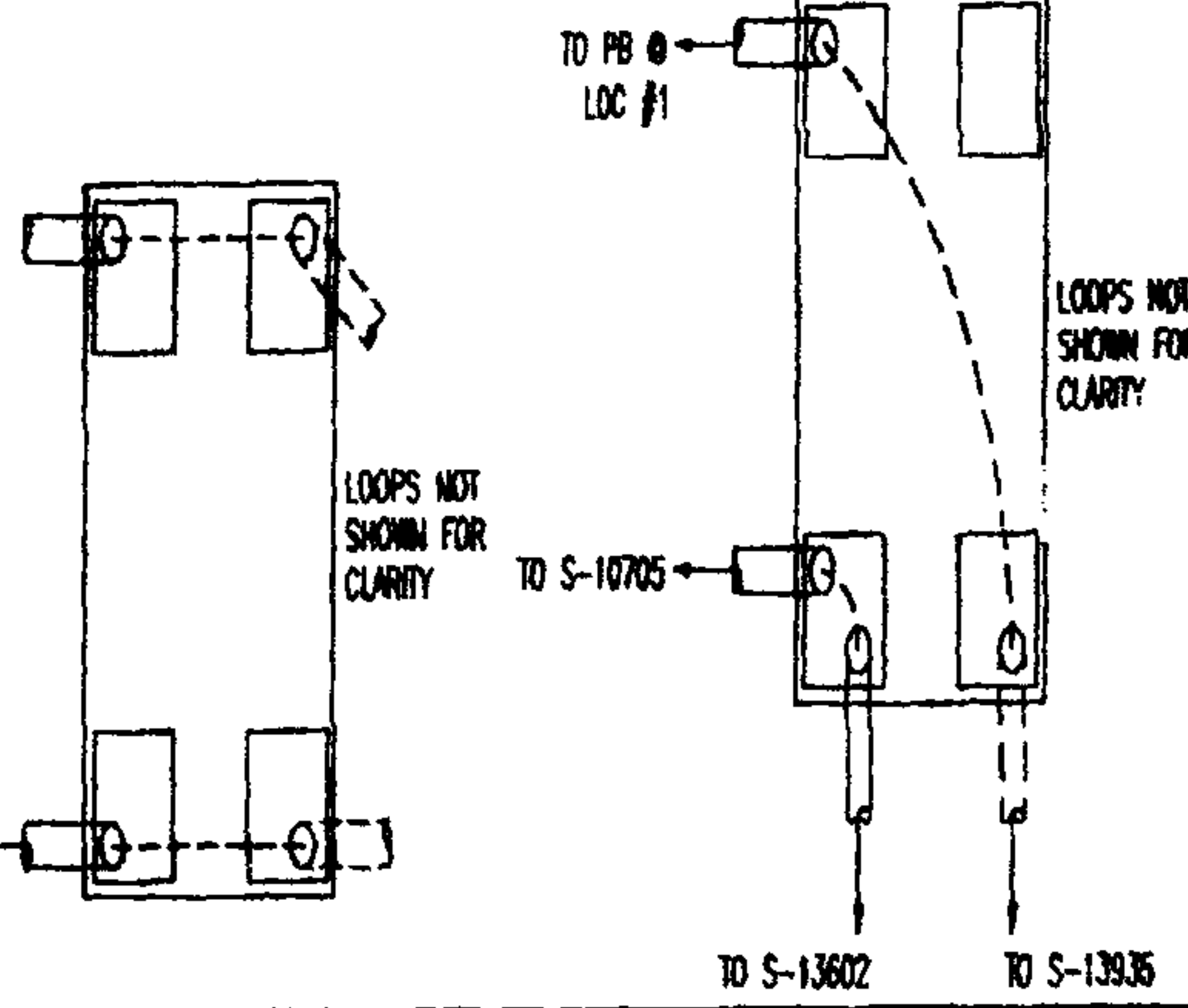
PULLING @ LOCATION 16
