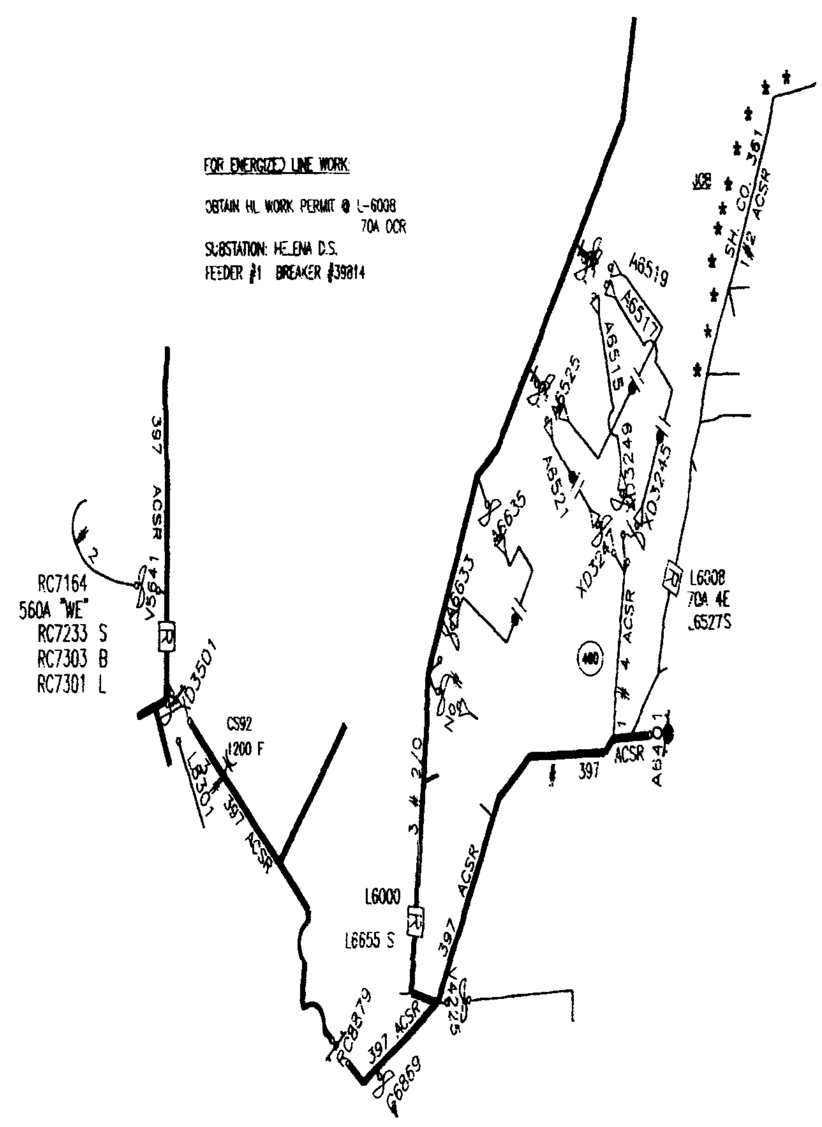
SECTIONALIZING SKETCH
