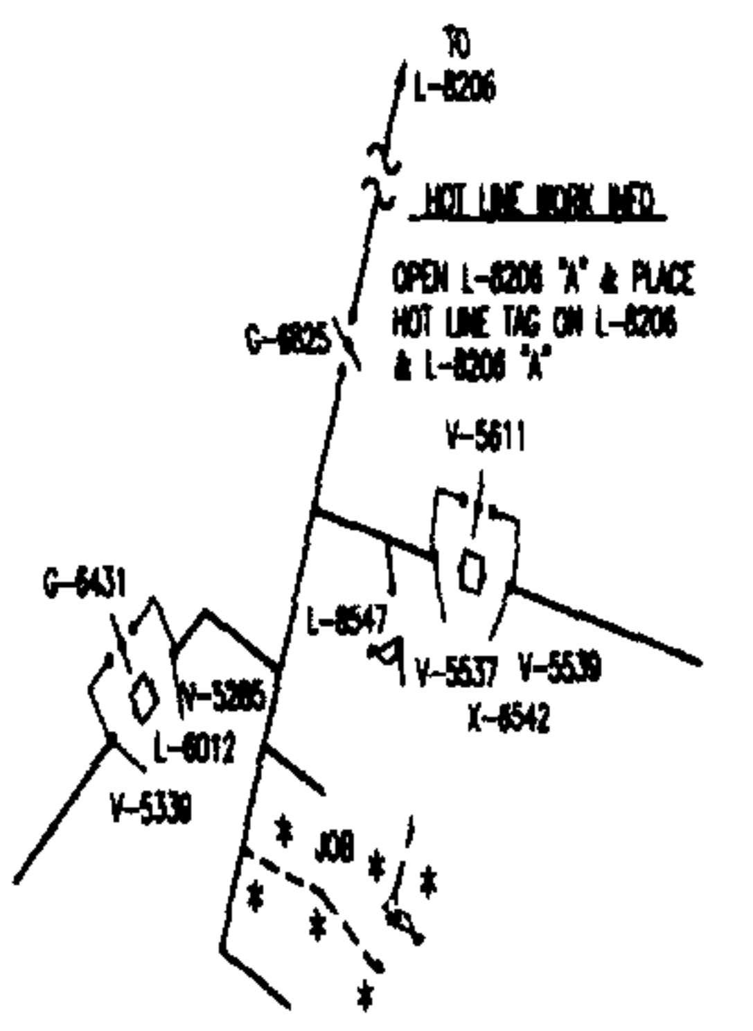
34.5KV SECTIONALIZING SKETCH
