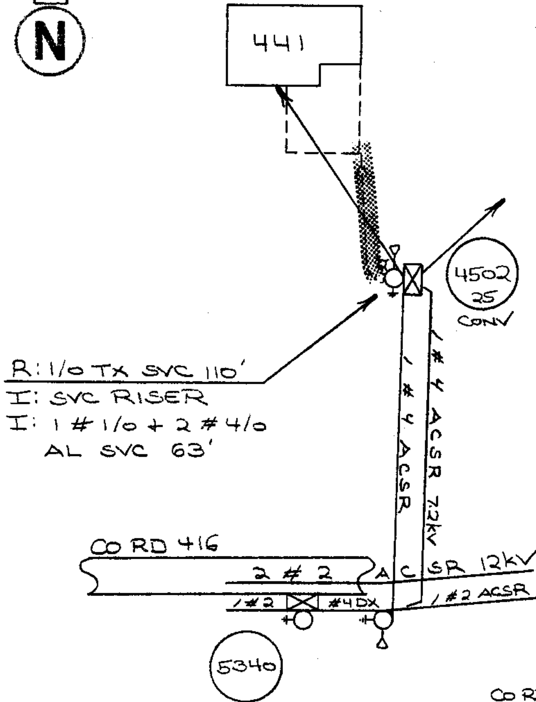
LOCATION SKETCH
